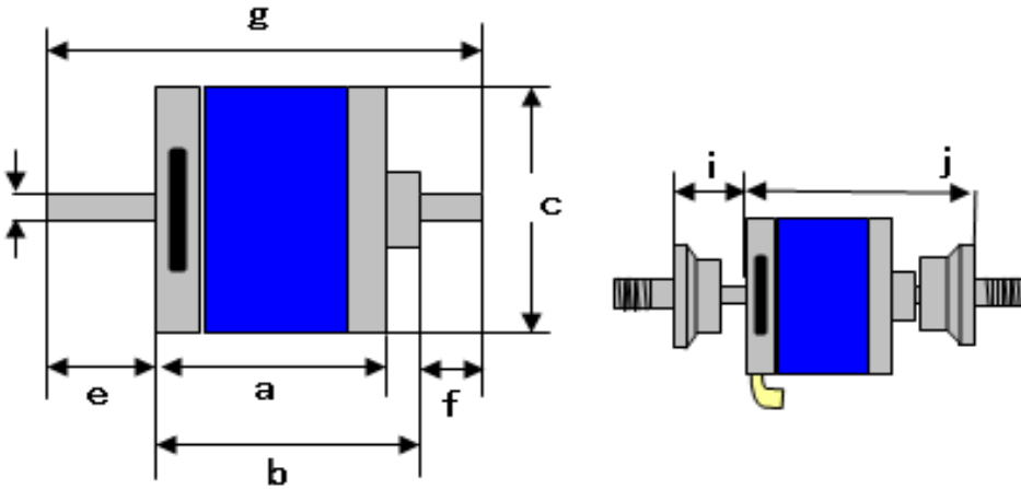
Zs22 series dimensions in millimeters (mm)
